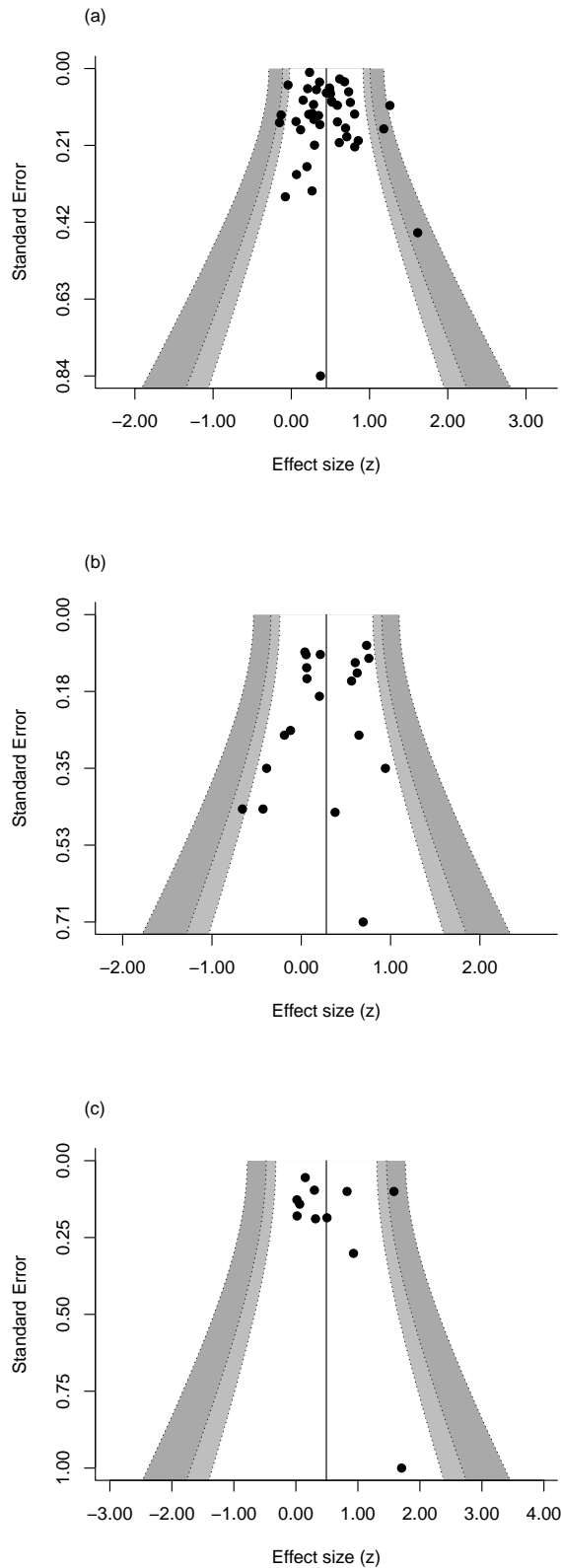
Figure S1: Contour-enhanced funnel plots showing the relationship between study effect size and standard error (study precision) for the relationship between range size and (a) habitat breadth, (b) diet breadth and (c) environmental tolerance range. Vertical line indicates the model estimate (mean effect size). Confidence intervals (white: 90%, light grey: 95%, dark grey: 99%) show statistical significance of study effect sizes.
