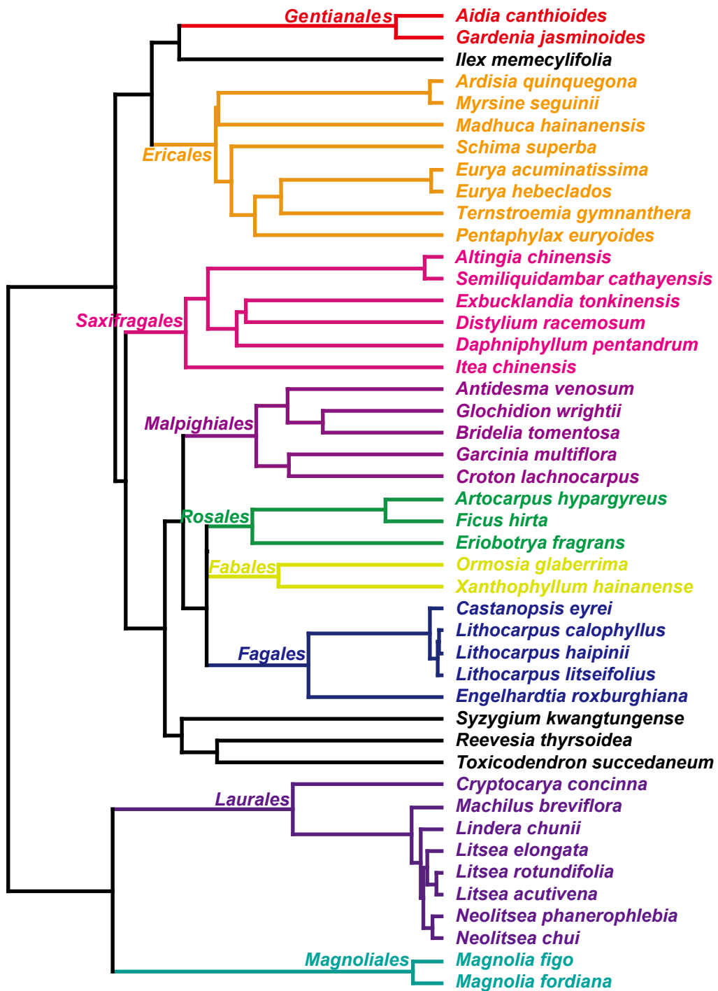
Figure S2. The maximum-likelihood phylogenetic tree of 45 plant species.
