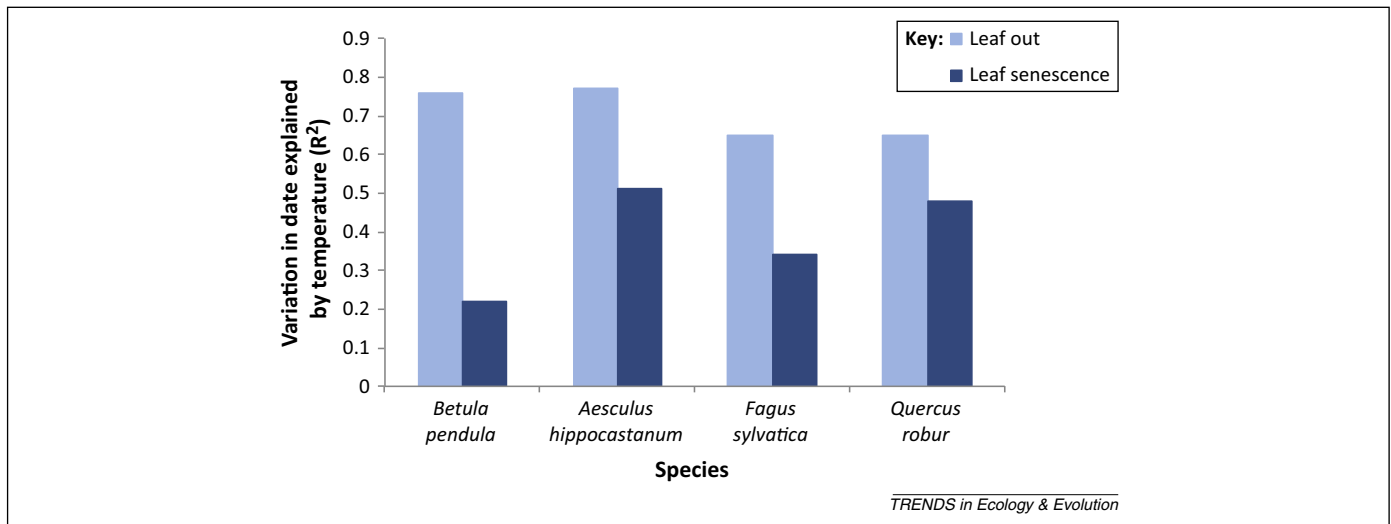
Figure 2. Temperature explains more variation in spring than in autumn leaf phenology. Correlation coefficients ( R^2 ) between event date and the preceding mean monthly spring and autumn temperatures for four tree species in Germany (1951–2000). Data from [15].
