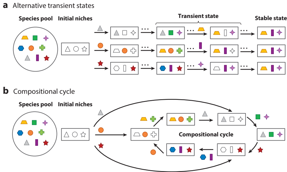
Figure 3 Schematic representation of (a) alternative transient states and (b) the compositional cycle. Symbols are as in Figure 2.
